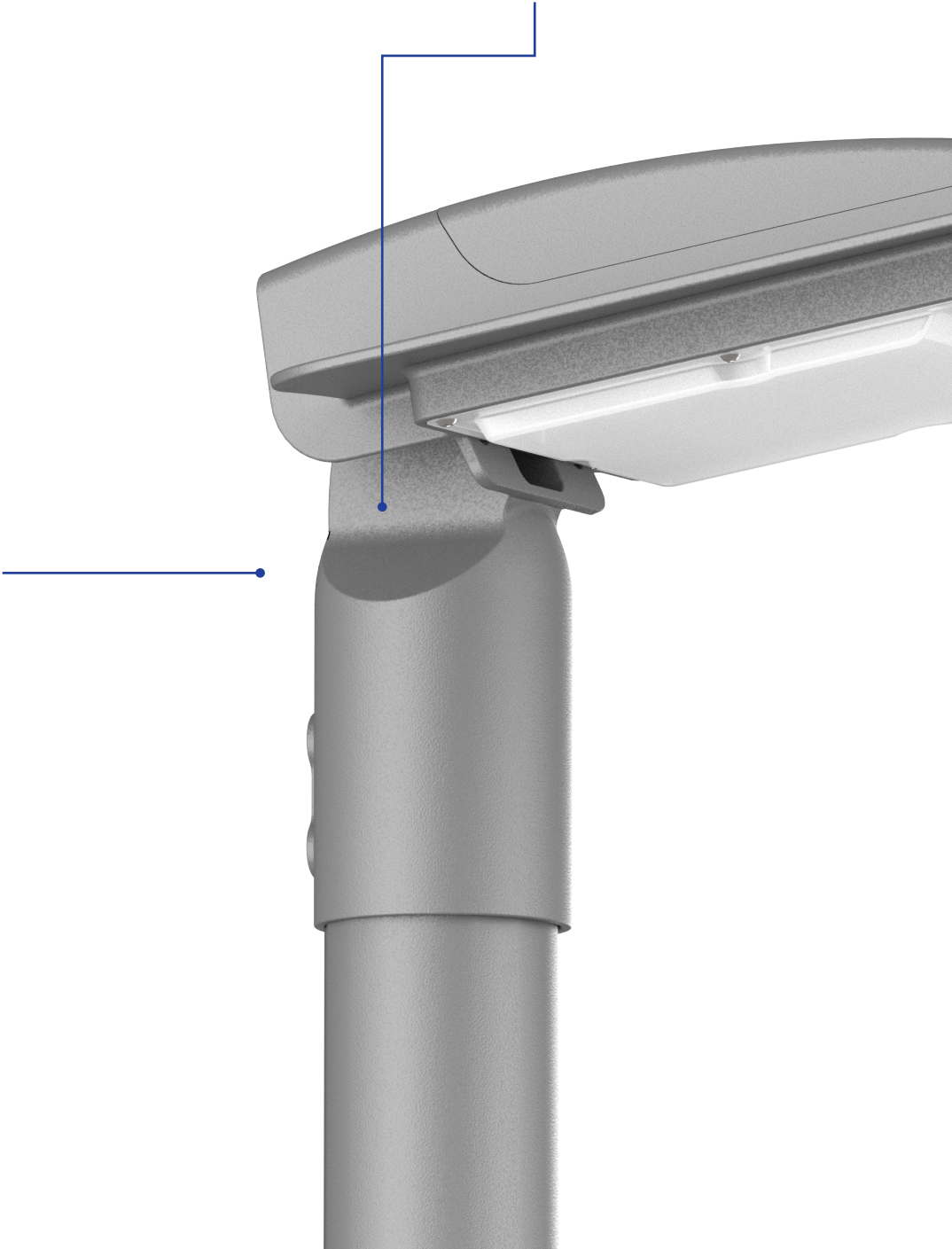
B type base can be adjusted by \pm 15 degrees. The lamp pole has a diameter of 60mm and is suitable for various installation environments.
